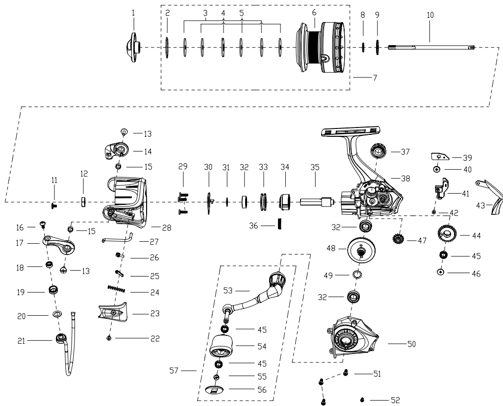
PARTS LIST OF MAXZSP30/40
